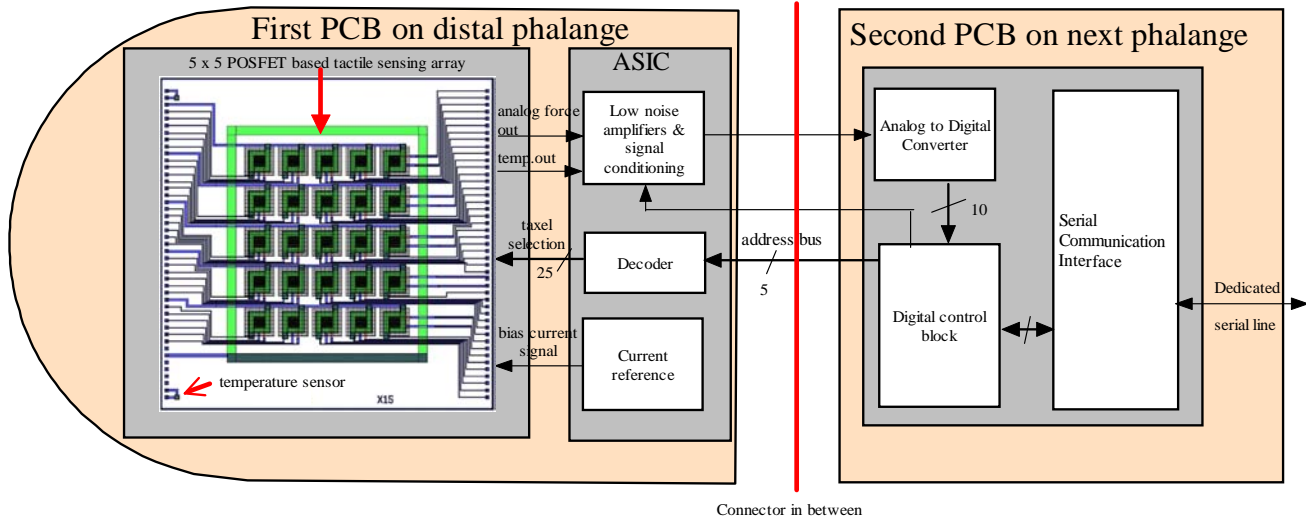
Fig. 3: System architecture (first phase) of tactile sensing system. The tentative location of different chips of the robot finger is also shown.
