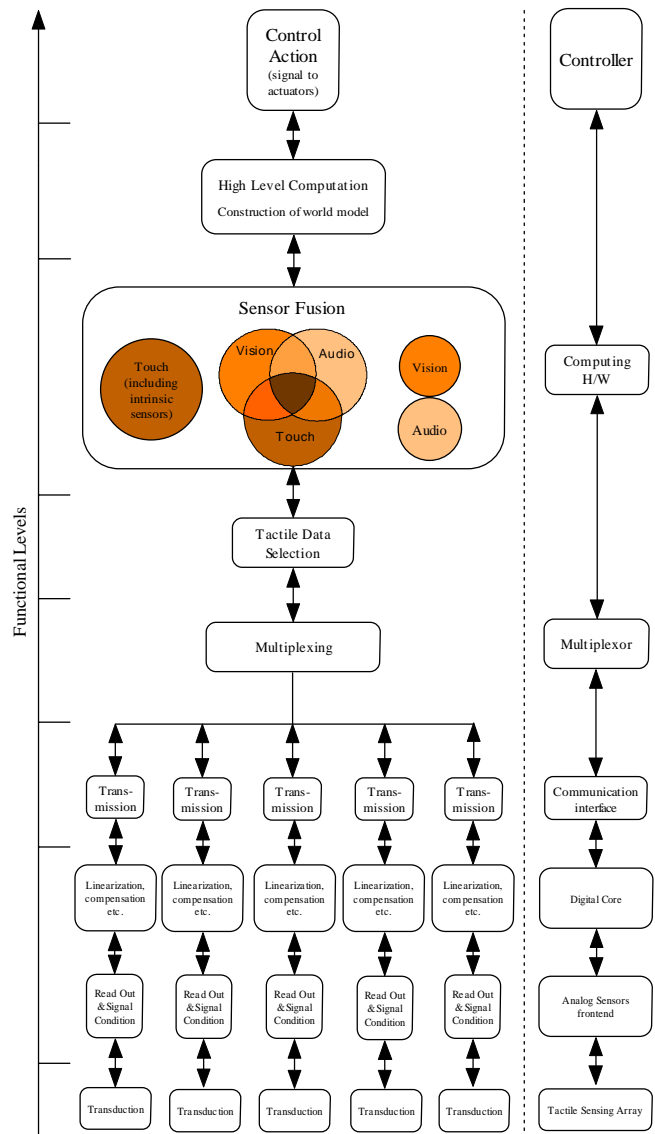
Fig. 1. Hierarchical functional and structural block diagram of Robot tactile sensing system.
